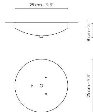
Canopy
