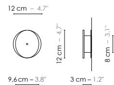
Wall plate
